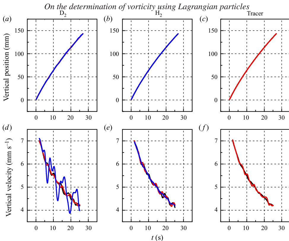
Figure 13. Temporal evolution of the ring vertical position ( a–c ) and velocity ( d–f ) obtained from the HVBK simulation. Panel disposition and line colour code as in figure 12 . Note that here, for the sake of clarity and comparison, we plot the absolute values of ring position and velocity in a fixed coordinate system, not moving with the ring and coinciding with the moving frame of reference at the beginning of the simulation (in the coordinate system of figure 11 the ring is moving downward, in the negative direction). The velocity time limits are due to the Gaussian algorithm chosen for the velocity calculation ( Švančara et al. 2020 ).
